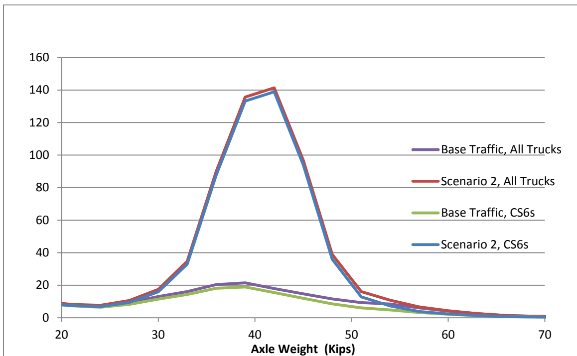
Figure 4: Scenario 2 Changes in Interstate Tridem Axle Loads
