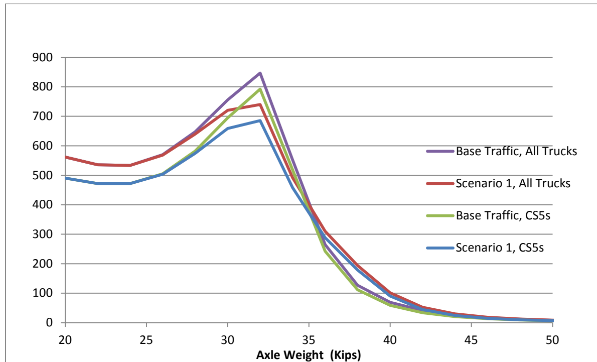
Figure 2: Scenario 1 Changes in Interstate Tandem Axle Loads
