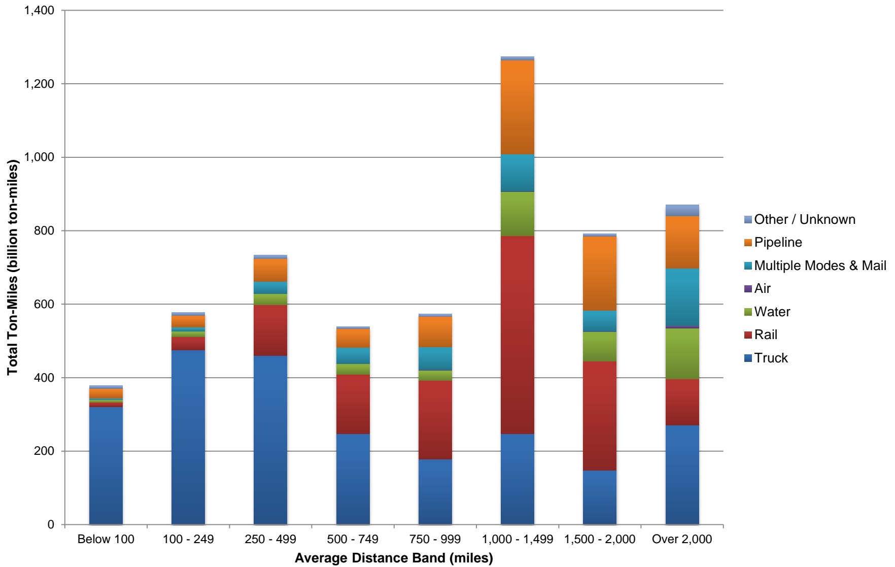
Figure 2-3b. Total Freight Ton-Miles by Distance Band: 2007
