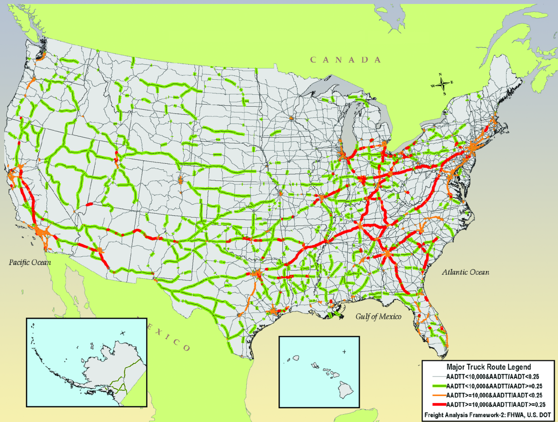
FIGURE 3-6. MAJOR TRUCK ROUTES ON THE NATIONAL HIGHWAY SYSTEM: 2002
