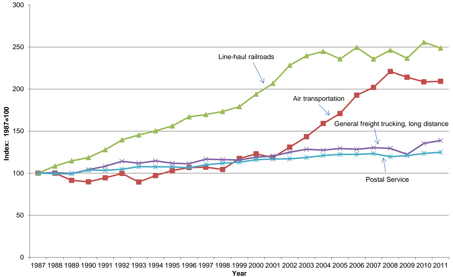
Figure 4-2. Productivity in Selected Transportation Industries: 1987-2011 (output per employee)
